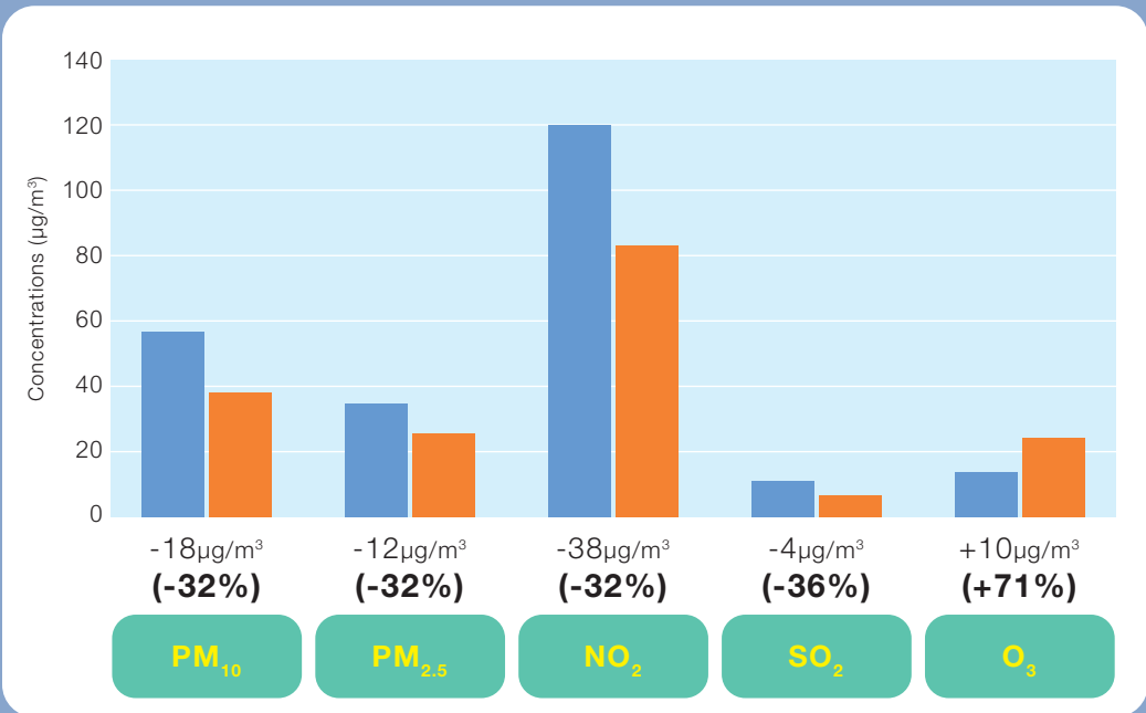
Figure 2: Changes in the concentrations of the key air pollutants at Roadside AQMS in Hong Kong from 2013 to 2018
