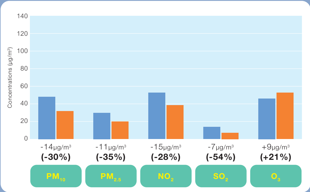
Figure 1: Changes in the concentrations of the key air pollutants at General AQMS in Hong Kong from 2013 to 2018
